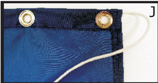
Eyelets: Standard 10mm Eyelet (inside Diameter) on a 30mm Hem with Cord.
